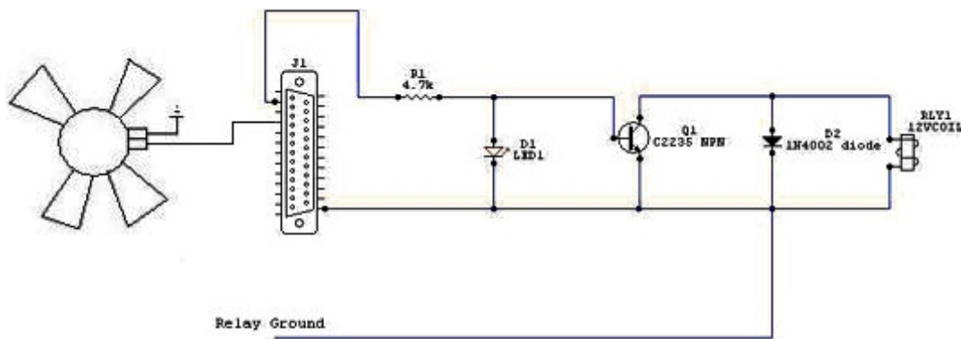
Fig. 4. Circuit to control home devices
